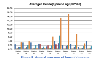
Figure 9. Annual averages of benzo(a)pyrene
