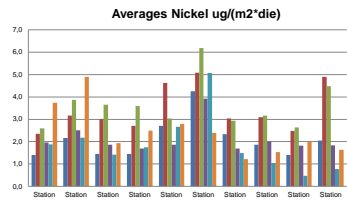
Figure 10. Annual averages of nickel
