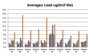
Figure 11. Annual averages of Lead
